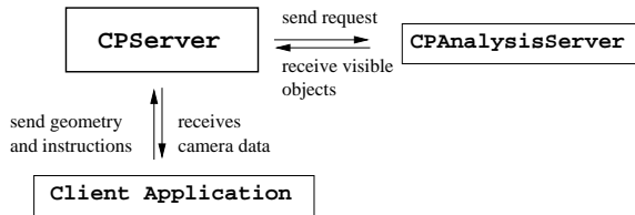
Figure 5: CubicalPath program structure
